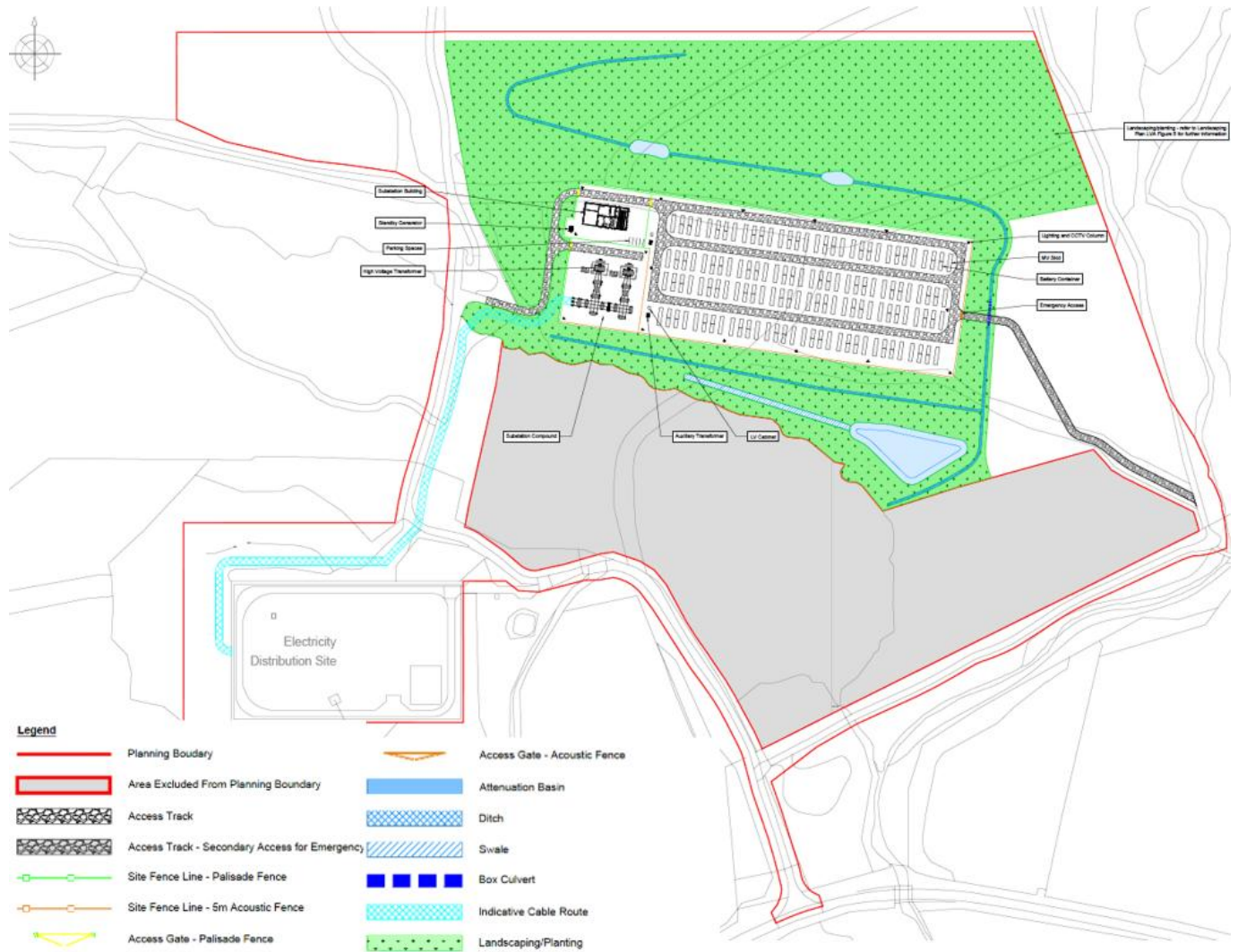
Figure 1: Indicative site layout for the Proposed Development
